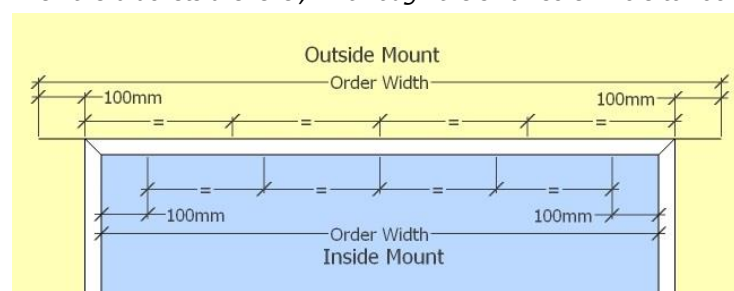
Bracket Mounting Positions
